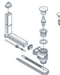
Basin adaptor
